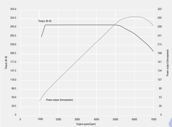
Portrait of an engineering masterpiece: the 335i/335i xDrive Advanced Turbo engine produces 300 hp at 5800 rpm, and quickly develops 300 lb-ft of torque at 1400 rpm, which continues without fading through to the 5000 rpm range. With such a broad range of powerful torque, you can enjoy smooth, robust acceleration in any gear, at any speed.
