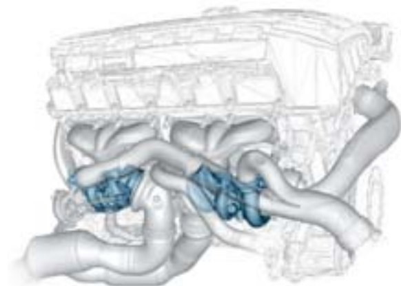
Fast buildup of pressure: the two parallel turbochargers (shown in blue) make a key contribution to the outstanding responsiveness of the 335i inline six-cylinder engine.
