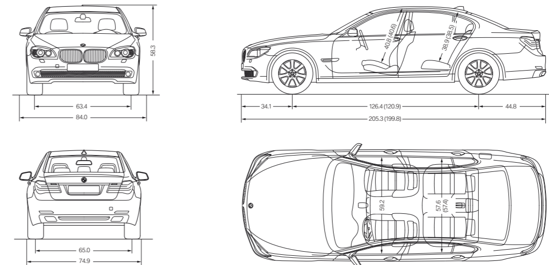
Technical drawing dimensions of 7 Series long-wheelbase models shown in inches. Figures in ( ) refer to the 740i, 750i (short-wheelbase version). ActiveHybrid 750i height is 58.5 inches; ActiveHybrid 750Li height is 58.4 inches. Height of 750Li and 750Li xDrive with roof antenna is 58.5 inches; 750i, 750i xDrive and ActiveHybrid 750Li height with roof antenna is 58.7 inches. Height of ActiveHybrid 750i with roof antenna is 58.8 inches; front track is 63.8 inches; rear track, 64.3 inches. Width at rear shoulder height in ActiveHybrid models is 57.4 inches.
