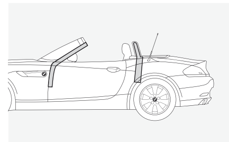
BMW's Rollover Protection System includes two steel roll bars behind the headrests and high-strength tubular steel integrated into the windshield support.
