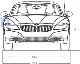
All dimensions in the technical drawings are given in inches for Z4 sDrive28i and Z4 sDrive 35i.
