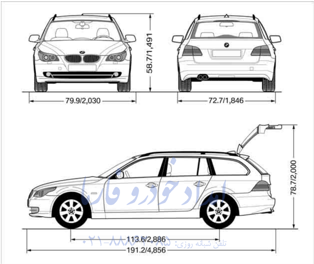
All dimensions given in inches/mm. Smallest turning circle diam.: 39 ft/11.9 m
